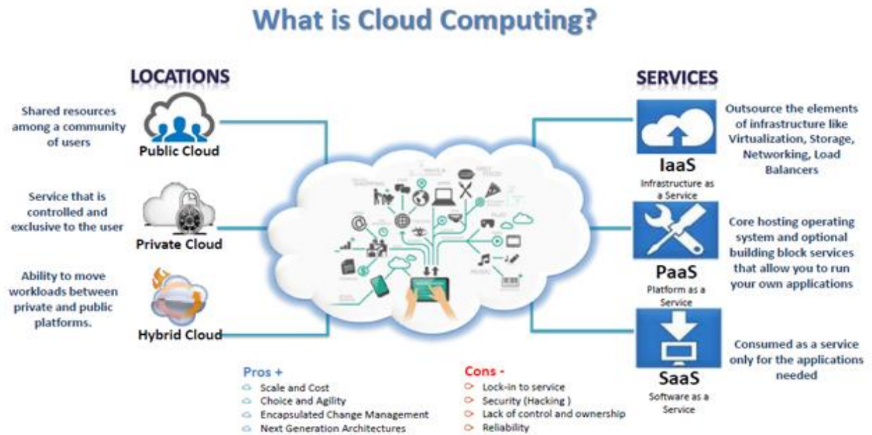
Fig 3.1: Cloud Computing
