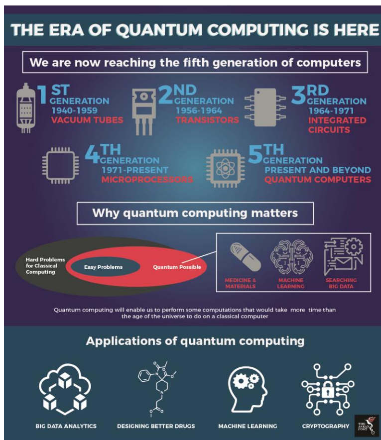
Fig 2.16: Quantum Computing
