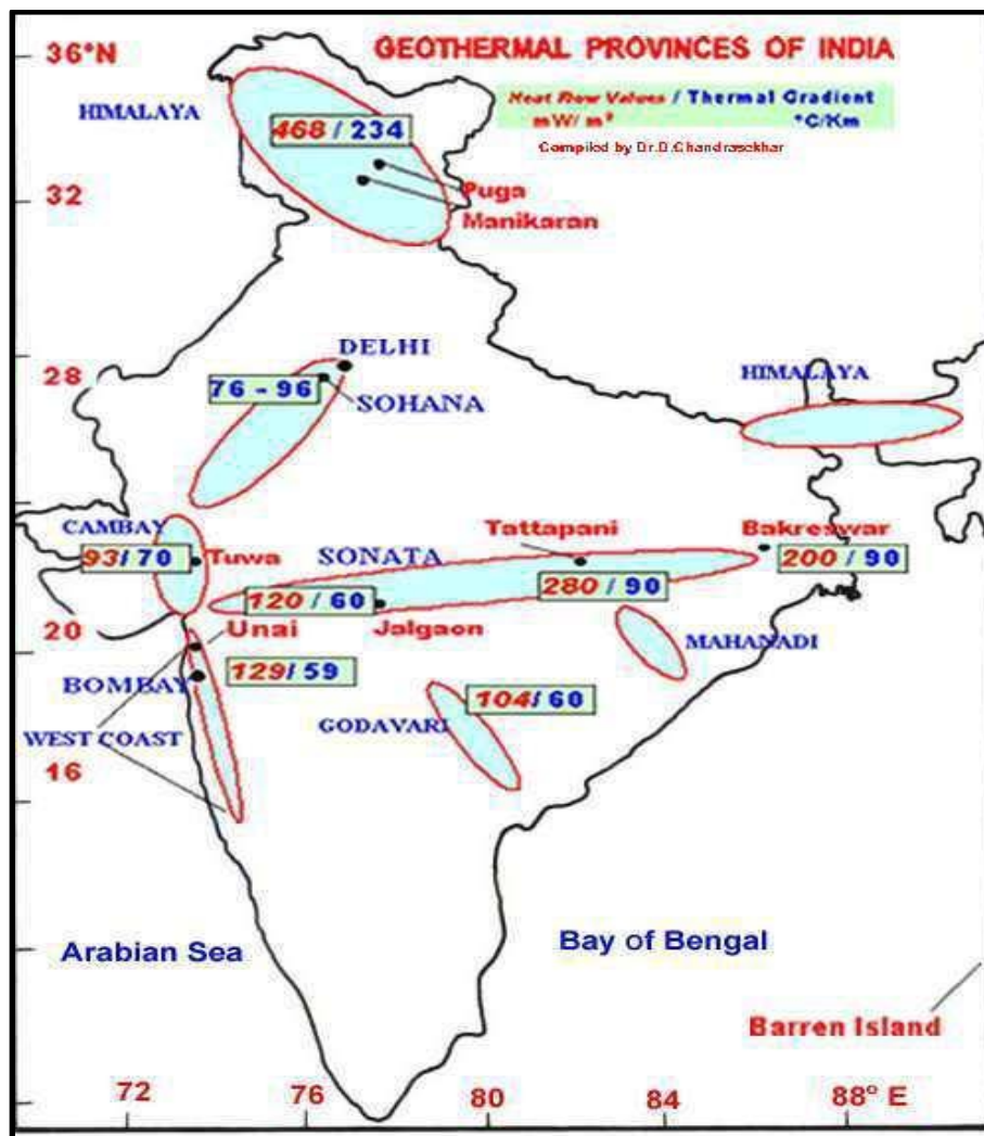
Fig 5.21: Geothermal Provinces in India
