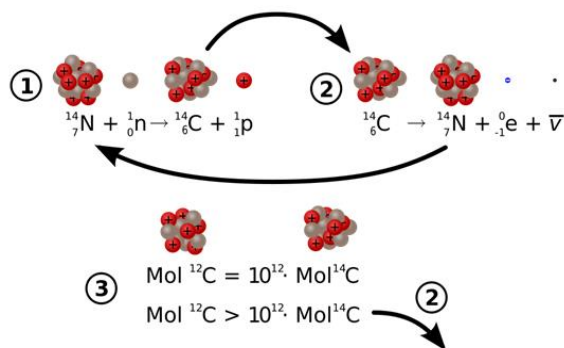
Fig 6.10 :Radiocarbon Dating
