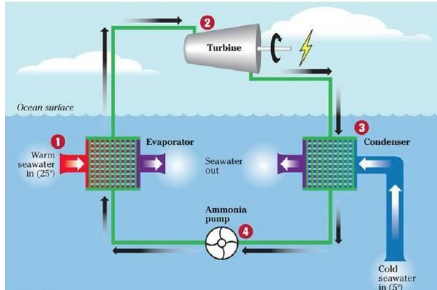
Fig 5.24-OTEC -process
